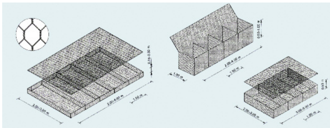
Figure n° 8 : gabions
