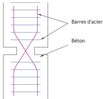
Articulation MESNAGER
