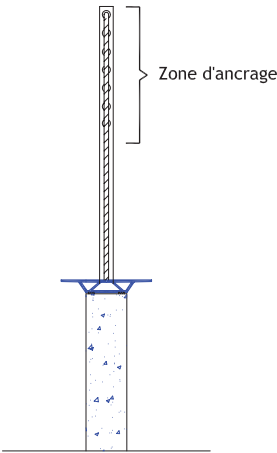
Haubanage axial
